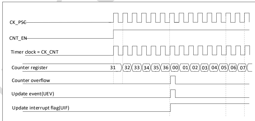
Figure 17-4 Counter timing diagram, internal clock divided by 1
