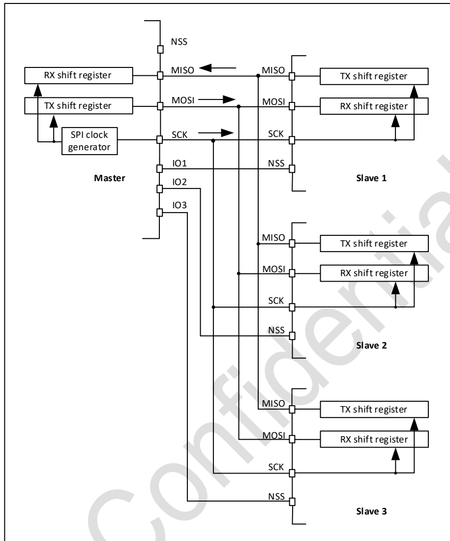
Figure 27-5 Master communicates with three independent slaves
