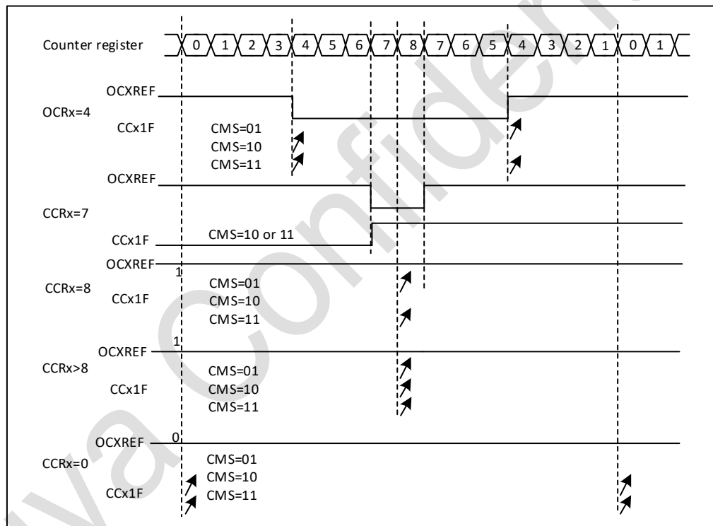
Figure 18-30 Center-aligned PWM waveforms (ARR = 8)
