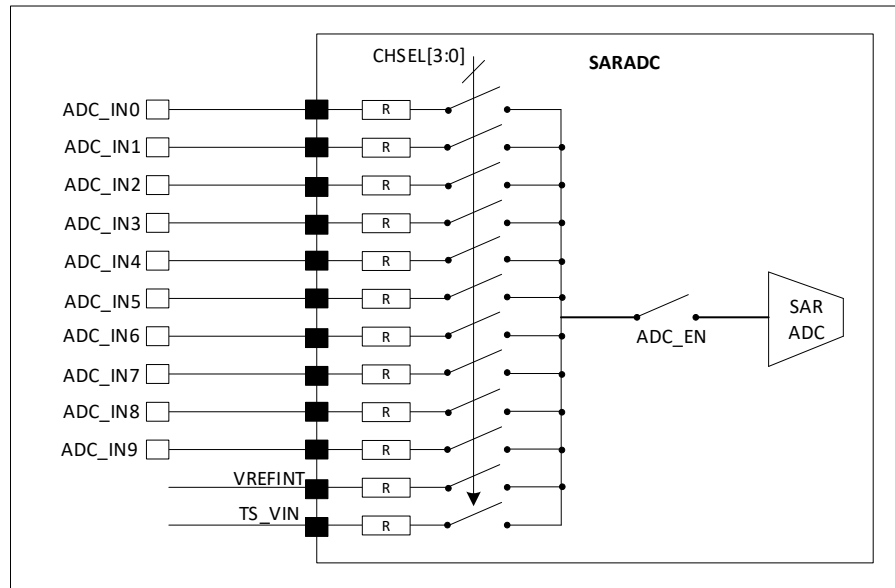
Figure 14-1 ADC channel with analog switch
