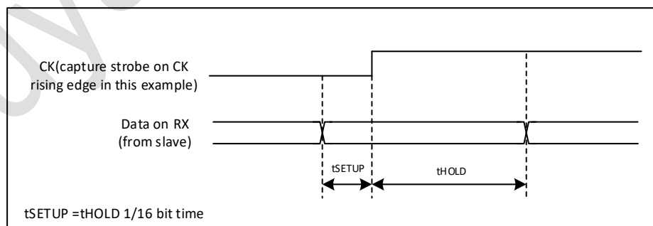
Figure 26-12 RX data sample/hold time
