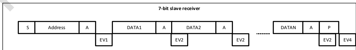
Figure 25-4 Slave receiver transmission sequence diagram
