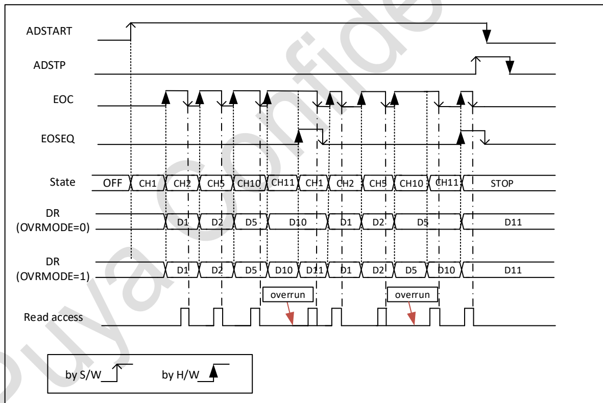
Figure 14-10 Overrun
