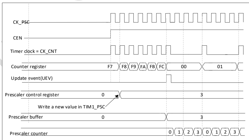
Figure 17-3 Counter timing diagram with prescaler division change from 1 to 4
