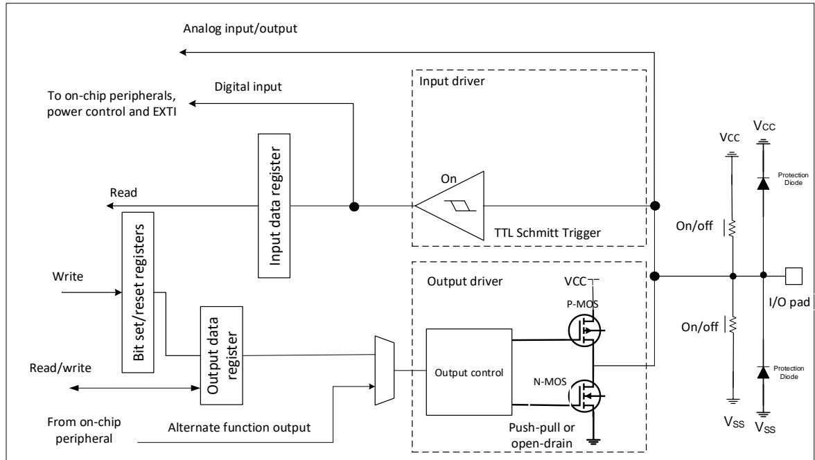
Figure 9-3 Output configuration
