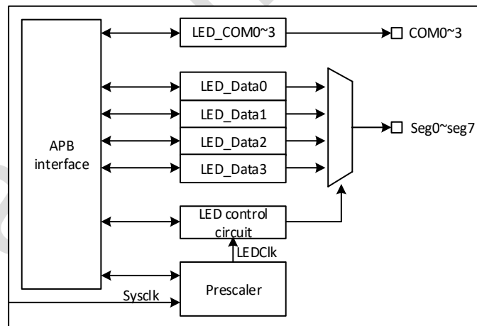
Figure 16-2 LED architecture diagram
