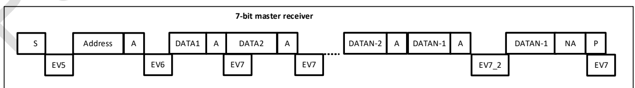
Figure 25-7 Method 2: Timing for master mode transmission when N > 2
