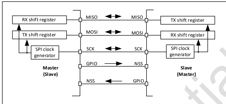
Figure 27-6 Multi-master application
