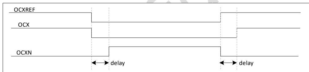
Figure 17-37 Complementary output with dead-time insertion
