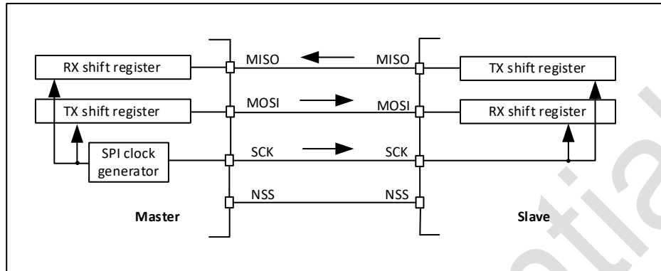
Figure 27-2 Full-duplex single master/slave application
