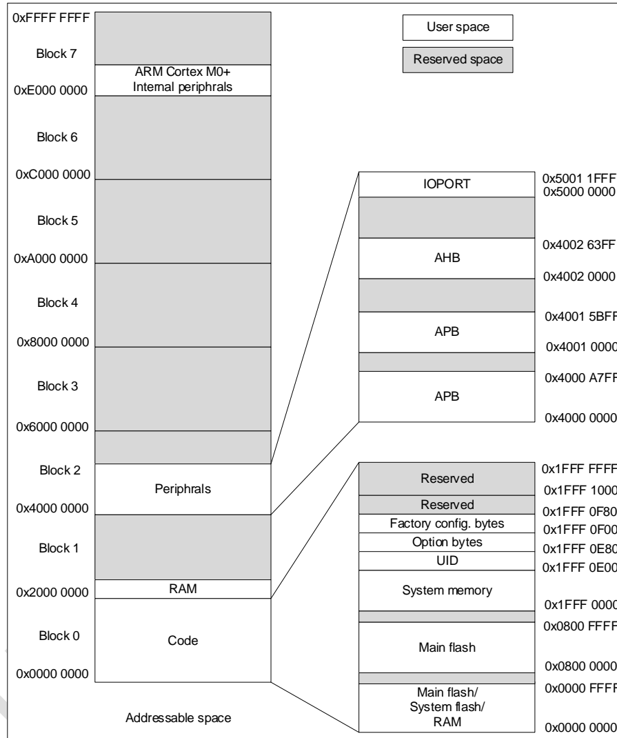
Figure 3-2 Memory map
