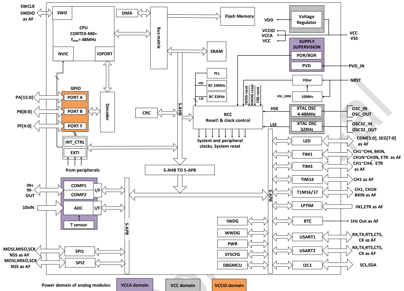
Figure 2-1 System architecture
