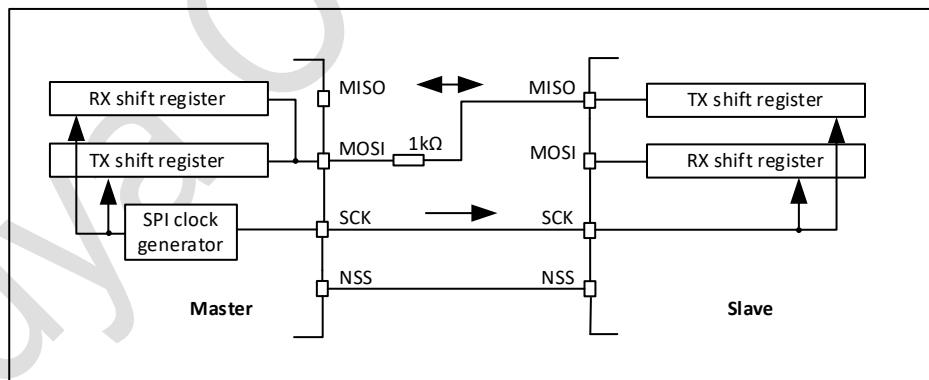
Figure 27-3 Half-duplex single master/slave application
