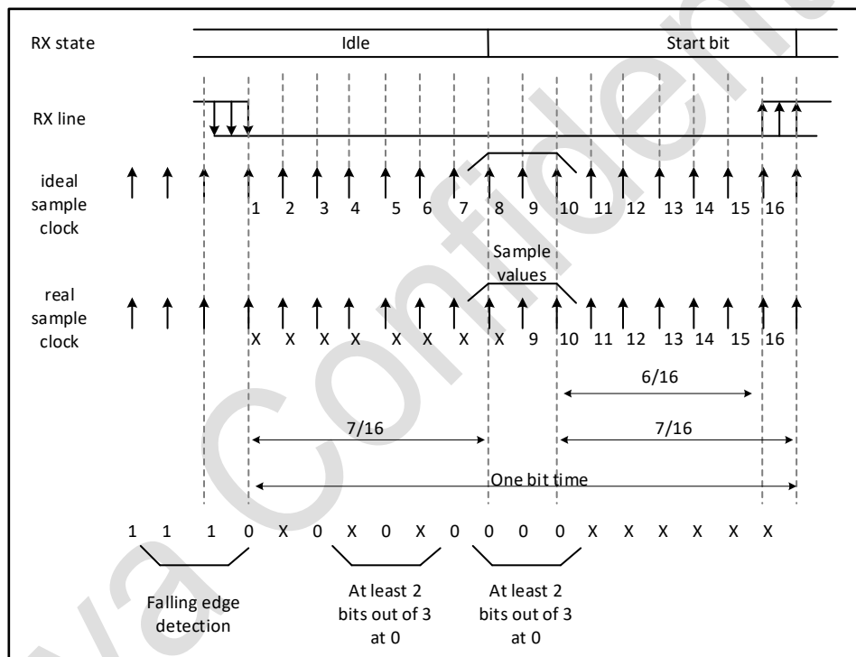
Figure 26-5 Start bit detection
